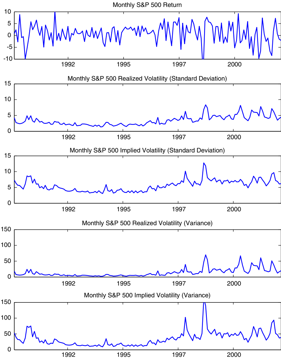
Fig. 1. Time series plot of returns and volatilities.
